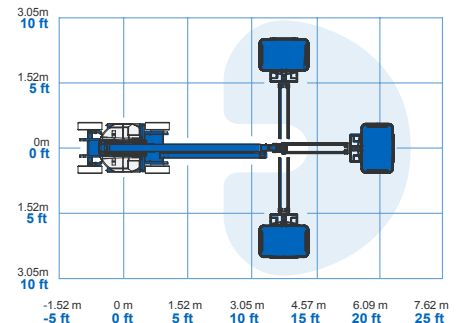
Jib Range of Motion Z-30/20N RJ
