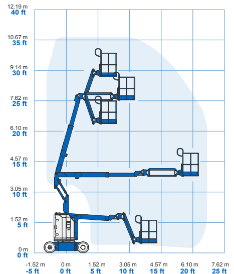
Range Of Motion Z-30/20N RJ
